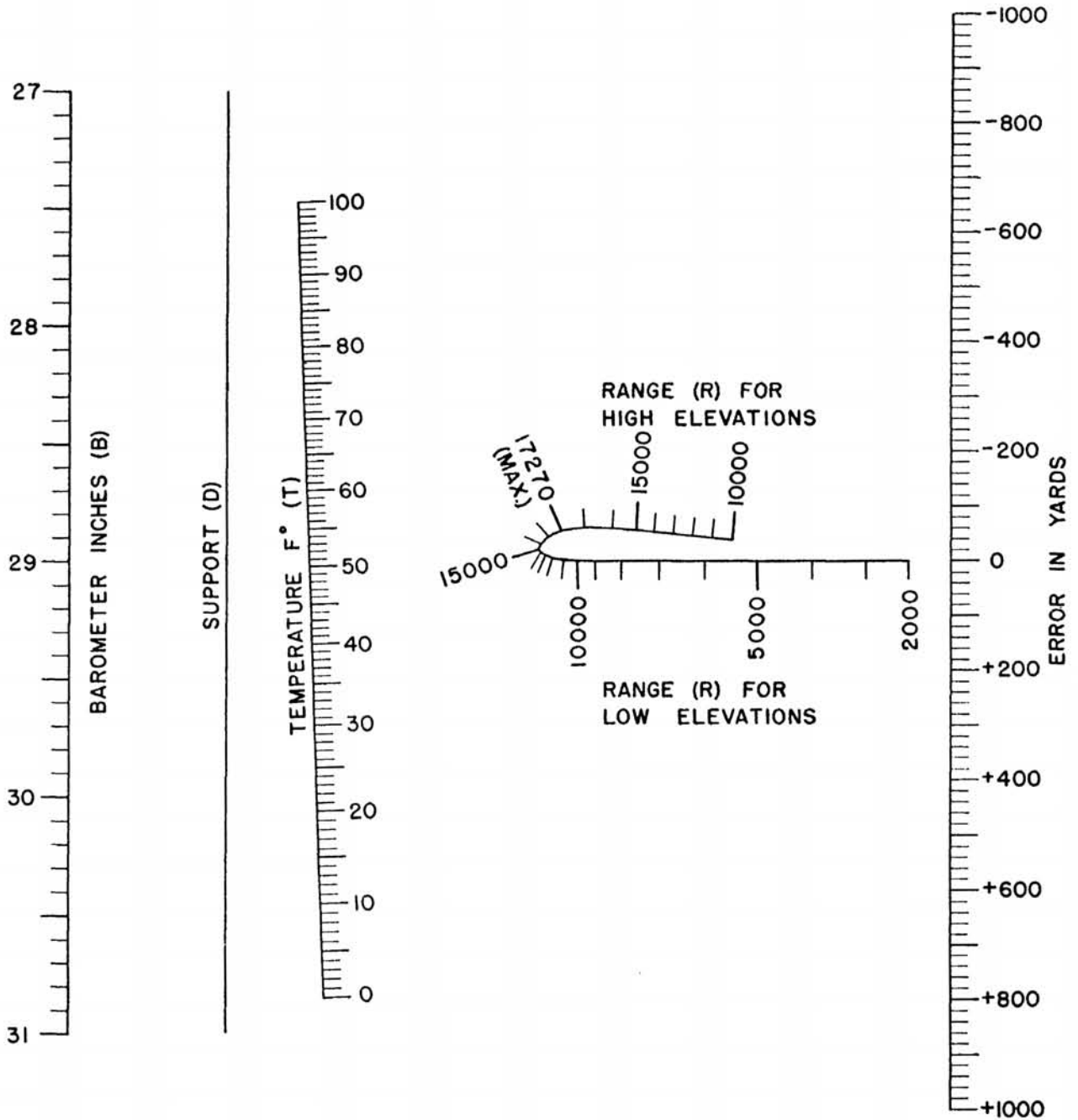
Figure 1.—Change in range for variation in density of air
